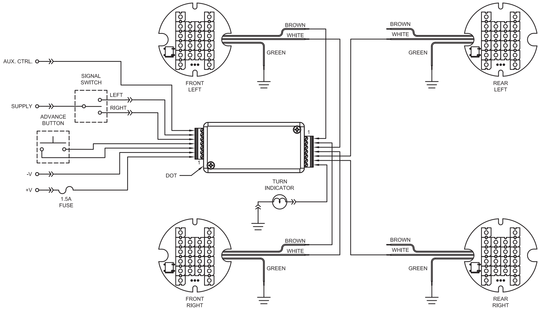
BTL4E-005 V2.0 HOOKUP DIAGRAM
